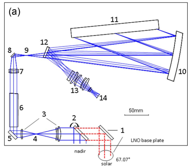
Fig. 6. Optical design of the LNO channel: (a) 2D top and (b) 3D bottom.
