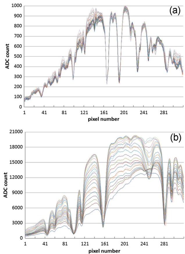
Fig. 37. Absorption spectra with SO [(a), order 160] and LNO [(b), order 168] of ambient air, registered with a broad infrared light source.
