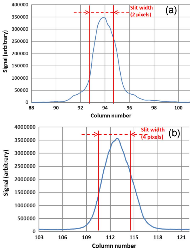
Fig. 34. ILP for detector row 132 [(a) SO] and averaged over 100 rows [(b) LNO] with slit illuminated by monochromatic laser light beam at 3.39 μm.
