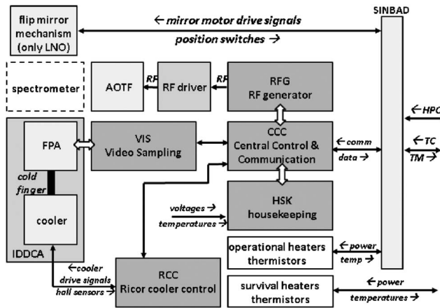
Fig. 21. Block diagram of electronics of SO and LNO channel.
