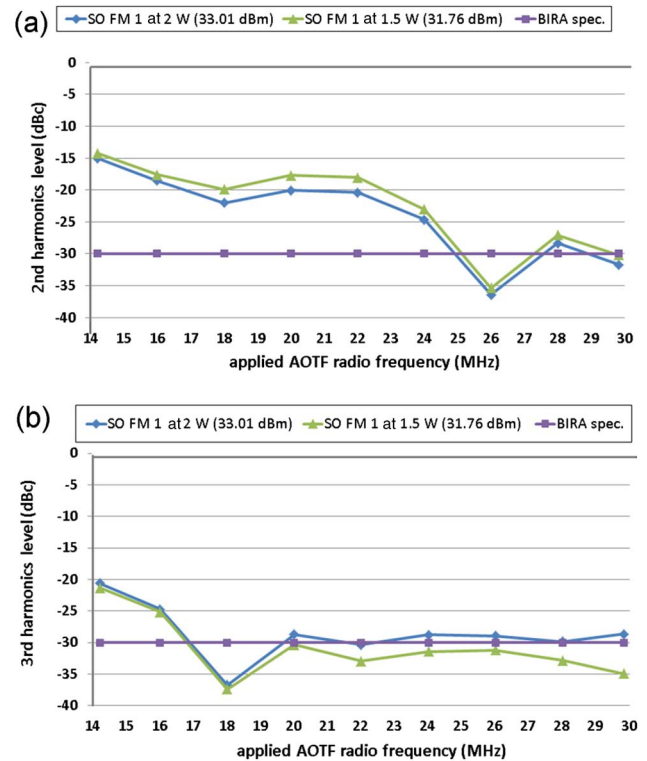
Fig. 22. (a) Second and (b) third harmonics levels of the radio frequency power amplifier (SO).
