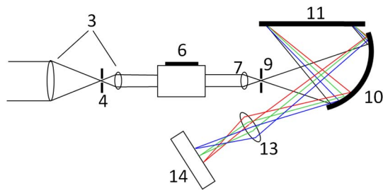
Fig. 4. Optical principle of NOMAD's infrared channels channel.
