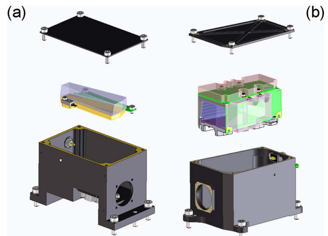
Fig. 14. Pictures of NOMAD AOTFs [(a): SO and (b): LNO].
