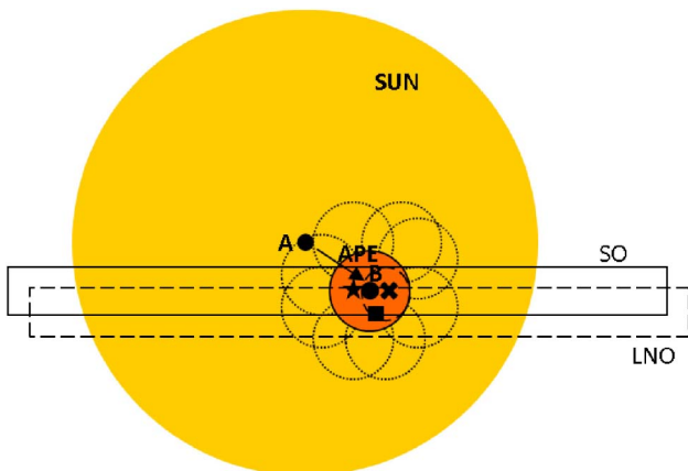
Fig. 2. NOMAD channel coalignment [A is center of the Sun; B is pointing axis of spacecraft; APE is absolute pointing error; full line rectangle is SO FOV; star is SO LOS; dashed line rectangle is LNO FOV; square is LNO LOS; dashed line circle is UVIS FOV; X is UVIS LOS; full line circle is maximum allowed misalignment between all LOS (including ACS); dotted targets are maximum allowed spacecraft RPE].
