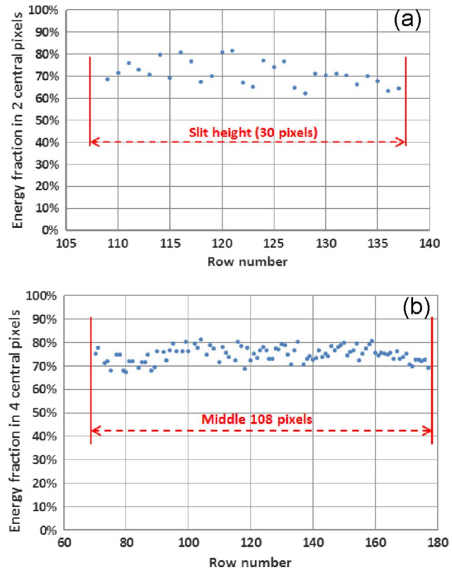
Fig. 35. Energy fraction in the two central pixels [(a) SO] and four central pixels [(b) LNO] over the slit height with monochromatic laser light beam at 3.39 μm.
