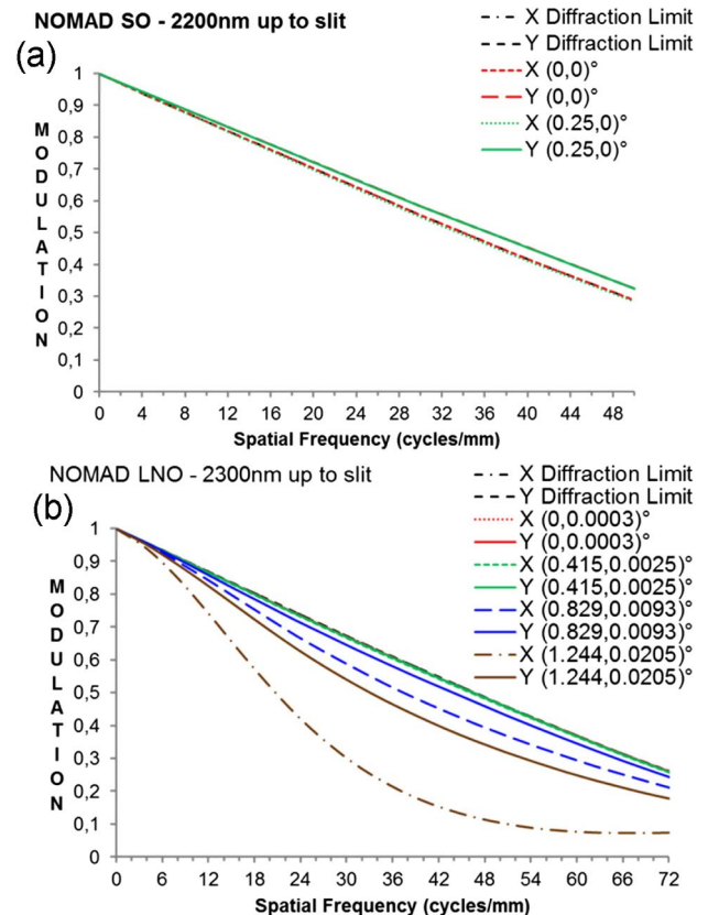
Fig. 30. MTF for optics in front of spectrometer slit. (a) SO, 2.2 \mu\text{m} and (b) LNO, 2.3 \mu\text{m} .
