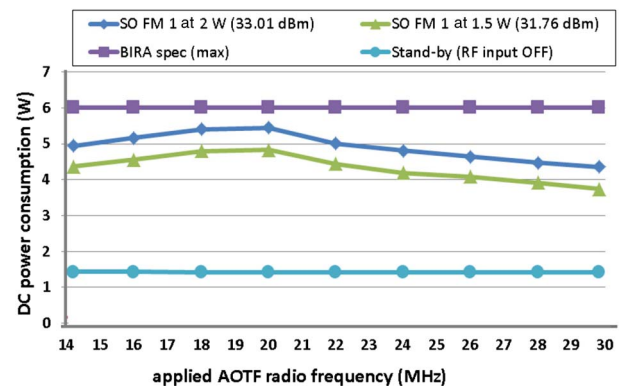
Fig. 23. DC power of the radio frequency power amplifier (SO).
