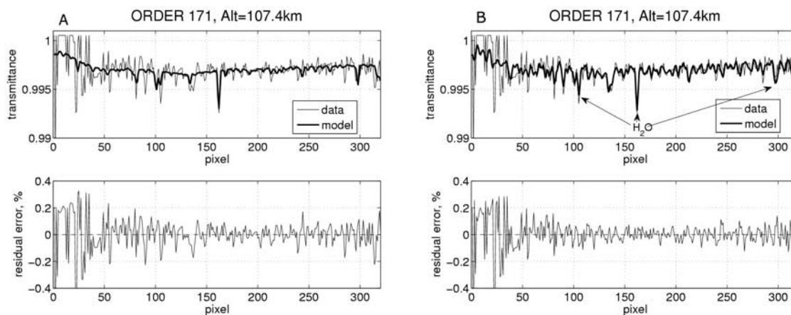
Figure 5. Contamination of adjacent orders in the main order 171 used for H 2 O retrieval. (a) \pm 3 orders around the main order have been taken into account. (b) \pm 6 orders around the main order have been taken into account. Those data were obtained during orbit 462 (27.07.2007) at the location latitude 87°N, longitude 245°E, 23.55 h Venusian local time (LT), distance to the limb 1830 km.
